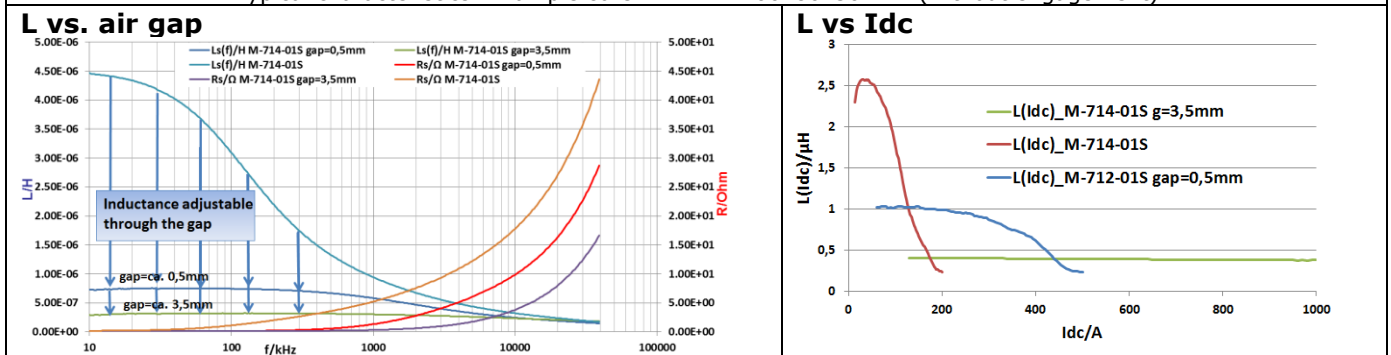
Typical characteristics: Example core M-714 = 100x80x30mm (without engagement)
