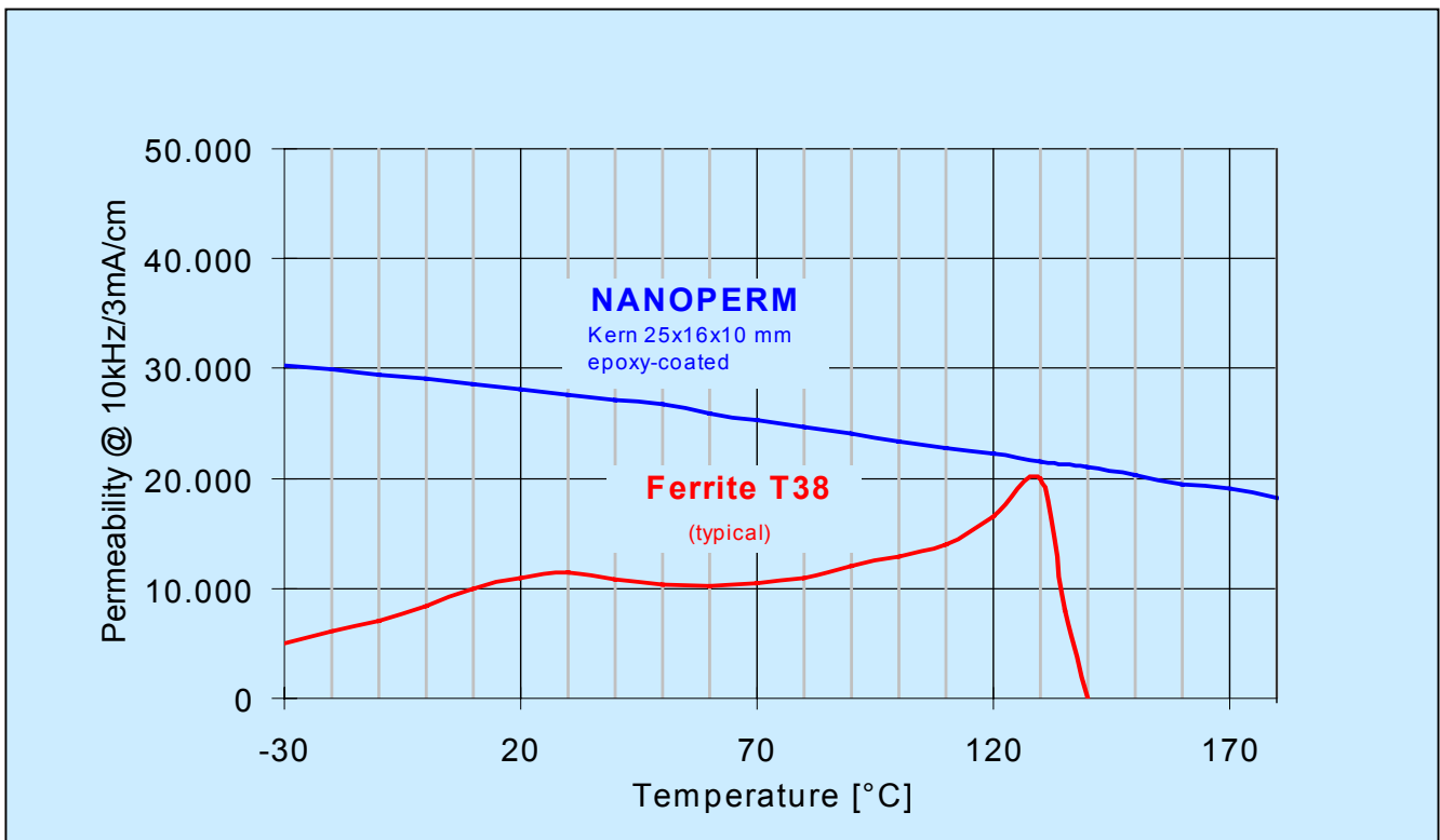
Permeability as a function of temperature
